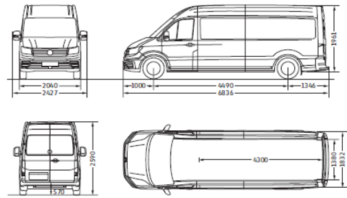
CR30/35 Panel van long wheelbase with high roof
